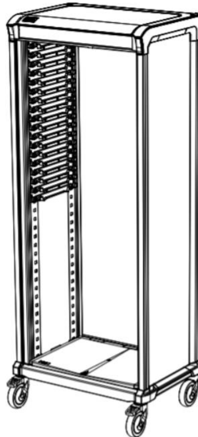
2. Combination of Panels & Telescopic Rails
